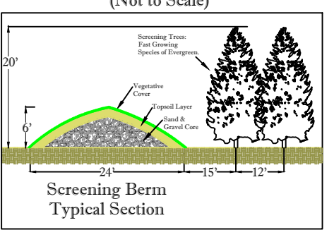
Perimeter Berms and Screening Trees (Not to Scale)
